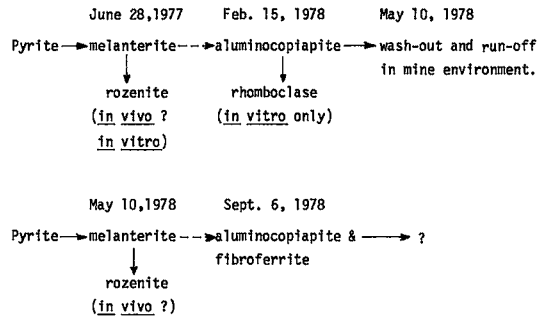
FIG. 5. Proposed alteration scheme for the formation of sulfates in the Prince mine. Dates of observations are shown above the mineral names. The broken arrow indicates that the formation of aluminocopiapite or fibroferrite and melanterite is conjectural.
