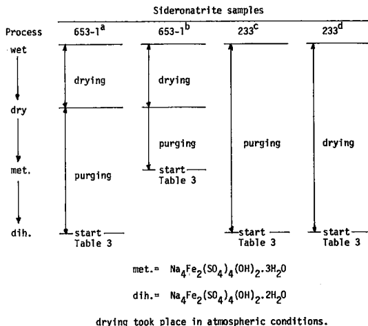
FIG. 2. Graphical illustration of dehydration behavior of samples of sideronatrinite or related products during pre-TGA in a dry N 2 atmosphere or in atmospheric conditions. Refer to Table 3.
