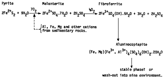
FIG. 4. Formation of hydrated sulfates from pyrite in #26 Colliery, 1-B mine. Broken lines indicate introduction of Al, Fe, Mg, etc. into the system. The step from fibroferrite to aluminocopiapite also requires an open chemical system.
